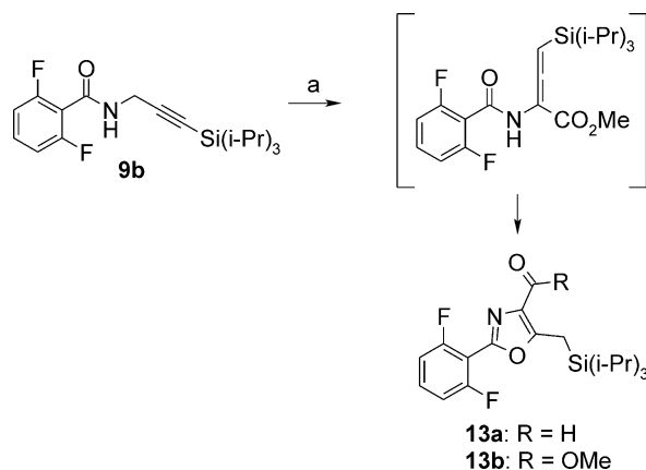
Scheme 4. Reagents and conditions: (a) 2.1 equiv n -BuLi, 2.2 equiv diisopropylamine, THF, -78^{\circ}\text{C} , then 1.1 equiv HCO 2 Et or ClC(O)OMe, 2 h, 50%.
