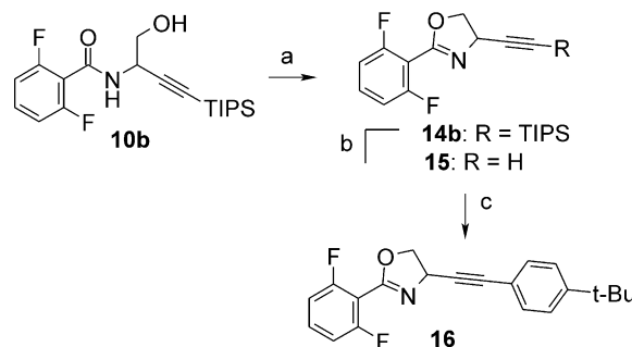
Scheme 5. Reagents and conditions: (a) 1.05 equiv Tf 2 O, pyridine, 15–20 ^{\circ}\text{C} , 0.5 h, 64%; (b) 1.2 equiv TBAF, 1.2 equiv HOAc, THF, 20 ^{\circ}\text{C} , 3 h, 88%; (c) 0.05 equiv Pd(PPh 3 ) 4 , 0.1 equiv CuI, 3.5 equiv NEt 3 , 2 equiv 4- t -butyliodobenzene, DMF, 20 ^{\circ}\text{C} , 14 h, 98%.
