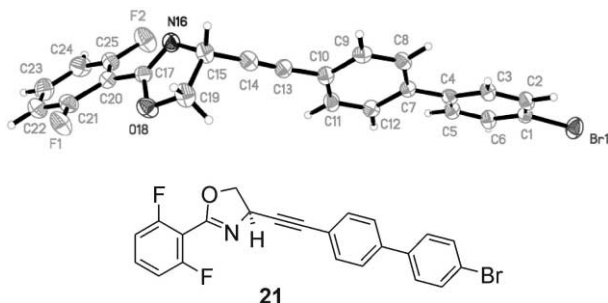
Figure 2. ORTEP representation of the X-ray crystal structure of compound 21 .
