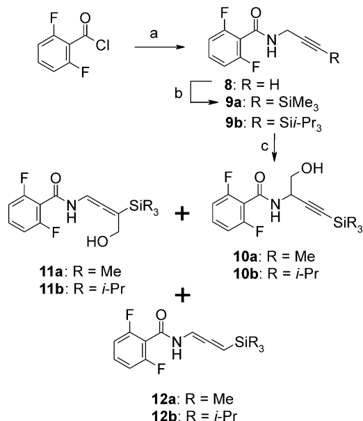
Scheme 3. Reagents and conditions: (a) 1.05 equiv propargylamine, 1.25 equiv NEt 3 , 0.01 equiv DMAP, CH 2 Cl 2 , 0–20 ^{\circ}\text{C} , 6 h, 97%; (b) 2.1 equiv n -BuLi, 2.2 equiv diisopropylamine, THF, -78^{\circ}\text{C} , then 1.1 equiv R 3 SiCl, -78 to 20^{\circ}\text{C} , 14 h, 85% for 9b ; (c) 2.05 equiv n -BuLi, 2.1 equiv diisopropylamine, 2.1 equiv TMEDA, THF, -78^{\circ}\text{C} , then excess CH 2 O(g), 0.5 h, 45% of 10b .
